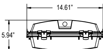
SVW4 - 4' Models
