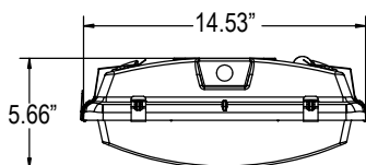
SVW2 - 2' Models
